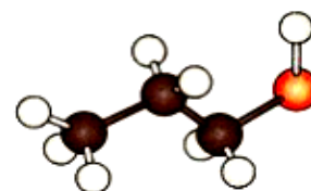
propan-1-ol
