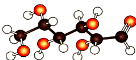
glucose
