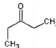
pentan-3-one
